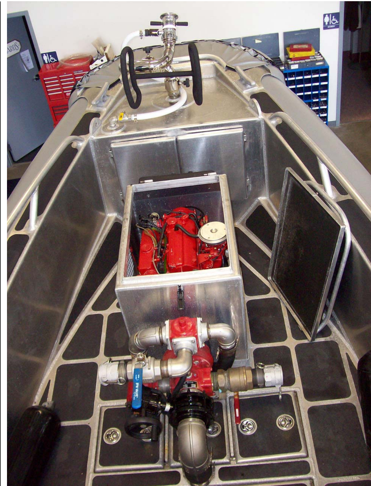
Fire Pump, Engine & Monitor with Foam Eductor Hose
